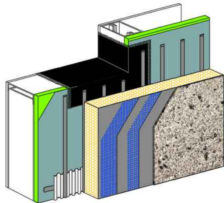
5A EFIS WALL CONSTRUCTION DRYVIT
